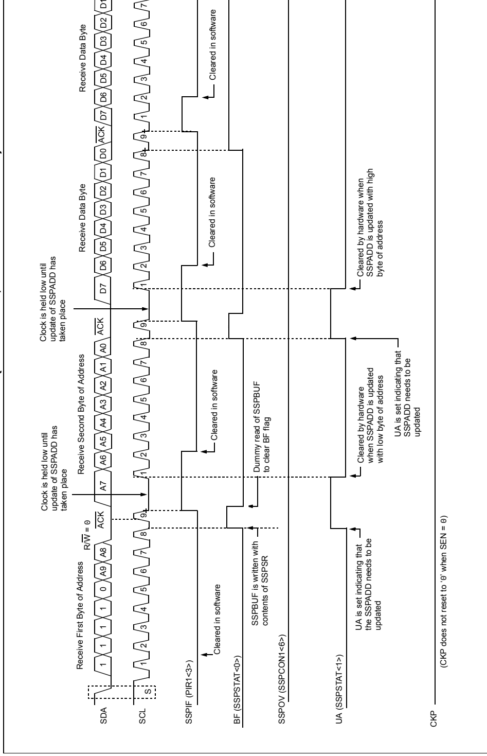
FIGURE 18-11: I 2 C SLAVE MODE TIMING WITH SEN = 0 (RECEPTION, 10-BIT ADDRESSING)
