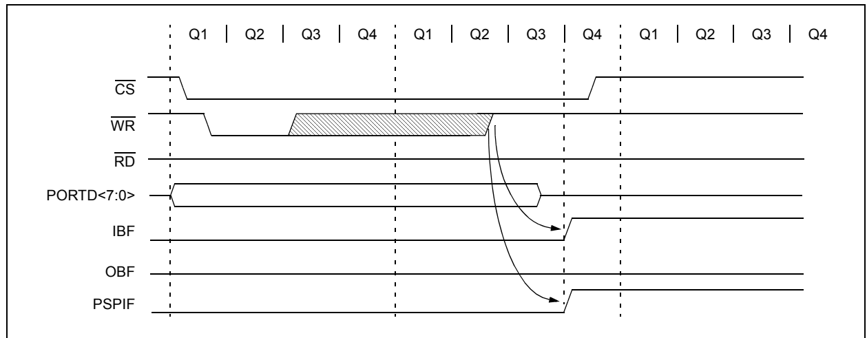
FIGURE 11-4: PARALLEL SLAVE PORT WRITE WAVEFORMS
