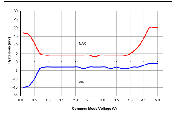
FIGURE 38-54: Comparator Offset, NP Mode ( CxSP = 1 ), V_{DD} = 5.0V , Typical Measured Values at 25^\circ C , PIC16F18857/77 Only.
