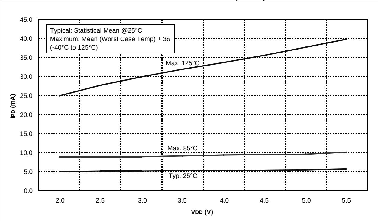
FIGURE 16-29: T1OSC I PD vs. V DD OVER TEMPERATURE (32 kHz)
