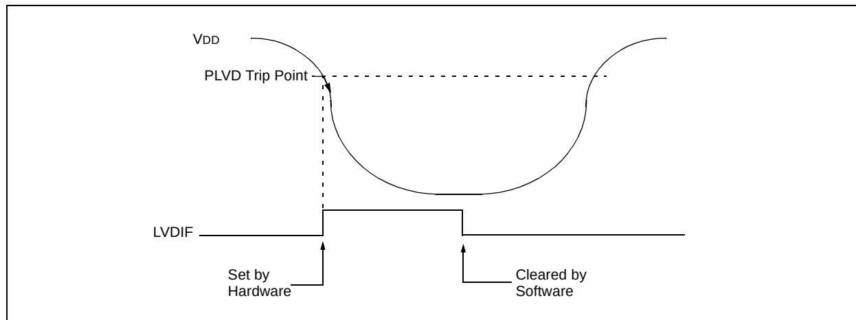
FIGURE 8-2: PLVD OPERATION
