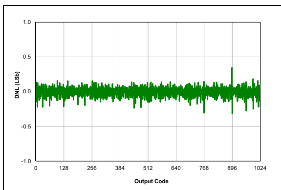
FIGURE 38-45: ADC, DNL, V_{DD} = 3.0V , T_{AD} = 1\text{ }\mu S , 25^\circ C .
