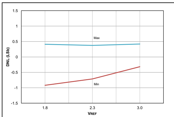
FIGURE 38-51: ADC 10-bit Mode, Single-Ended DNL, V_{DD} = 3.0V , T_{AD} = 1\text{ }\mu s .
