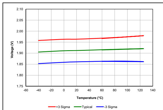
FIGURE 38-29: Brown-Out Reset Voltage, Trip Point (BORV = 11).
