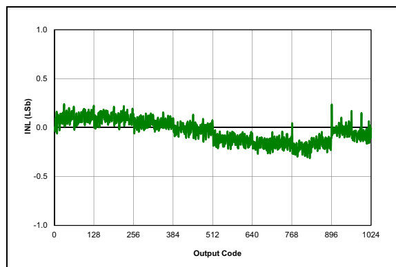
FIGURE 38-47: ADC, INL, V_{DD} = 3.0V , T_{AD} = 1\text{ }\mu S , 25^\circ C .
