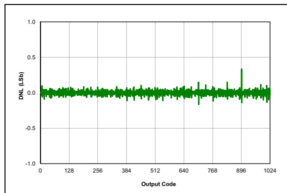
FIGURE 38-46: ADC, DNL, V_{DD} = 3.0V , T_{AD} = 4\text{ }\mu S , 25^\circ C .
