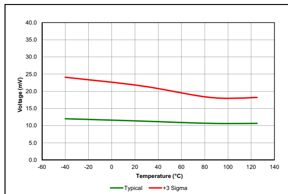
FIGURE 38-28: Brown-Out Reset Hysteresis, Trip Point (BORV = 1x).
