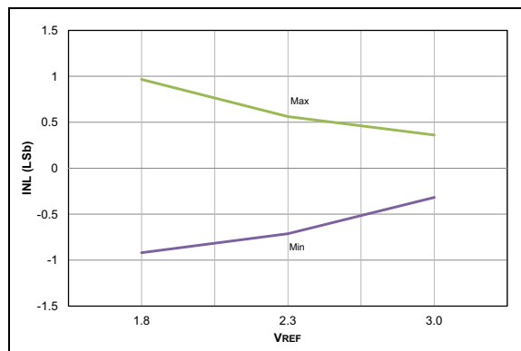
FIGURE 38-52: ADC 10-bit Mode, Single-Ended INL, V_{DD} = 3.0V , T_{AD} = 1\text{ }\mu s .
