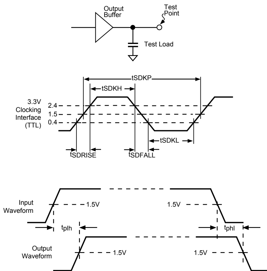
Figure 1. Clock Waveforms
