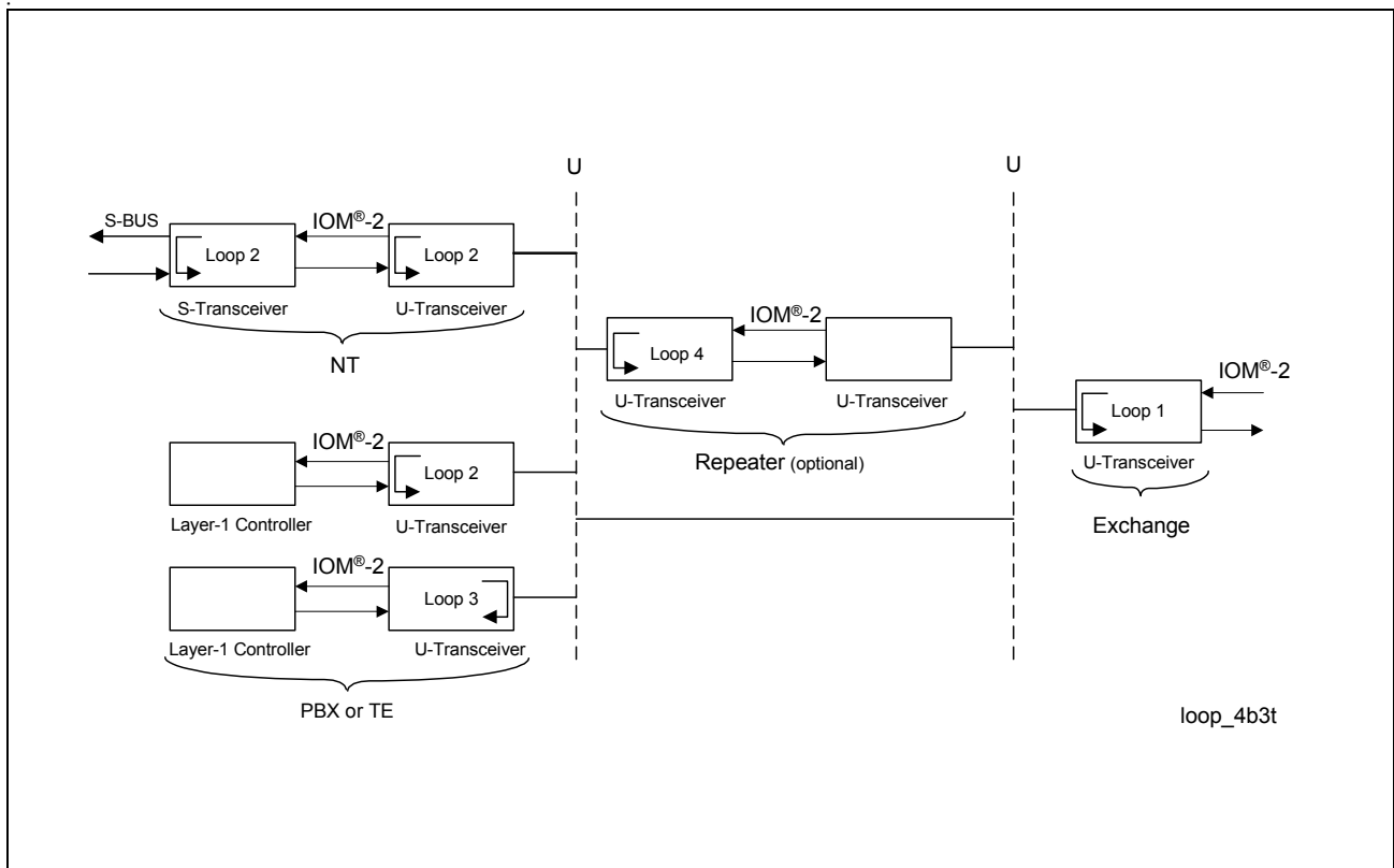
Figure 26 Test Loopbacks
