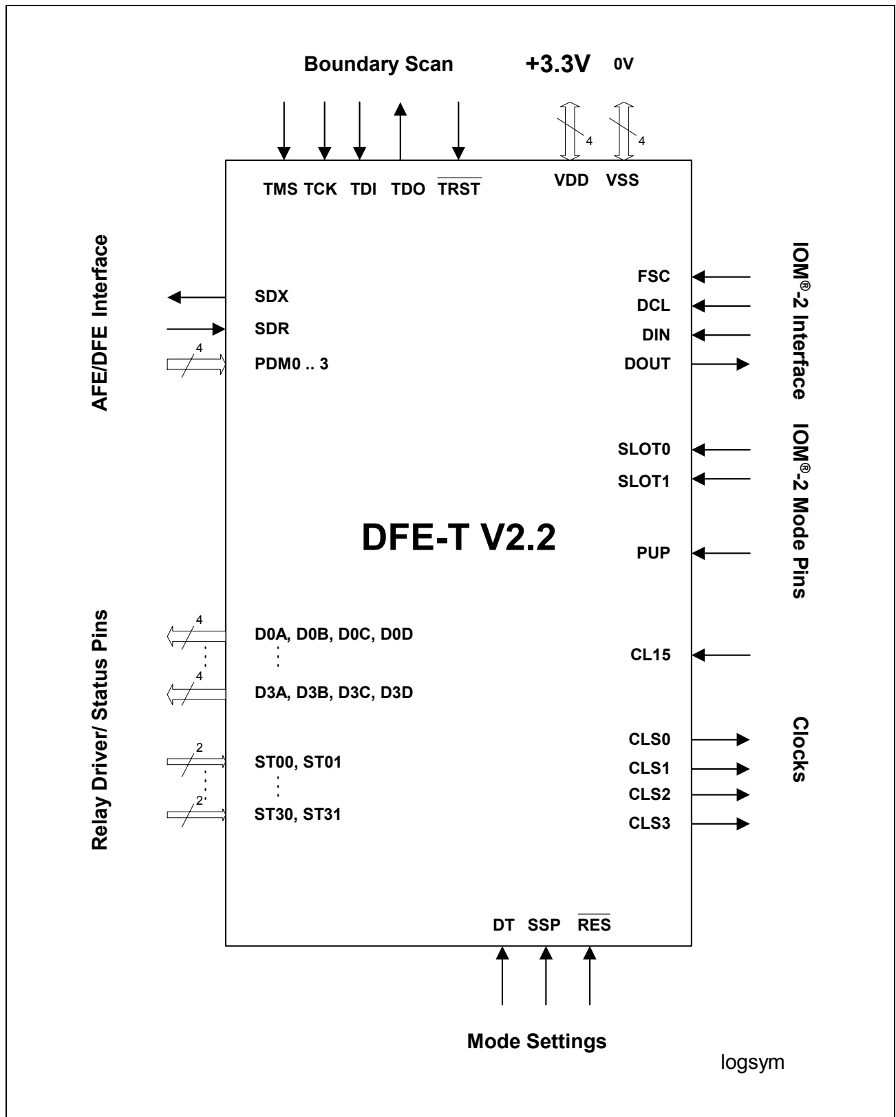
Figure 2 Logic Symbol
