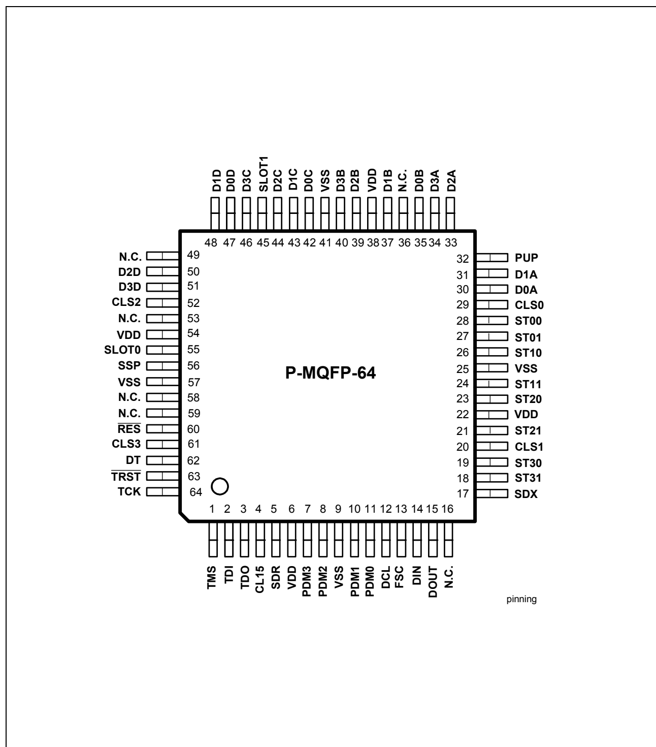
Figure 6 Pin Configuration
