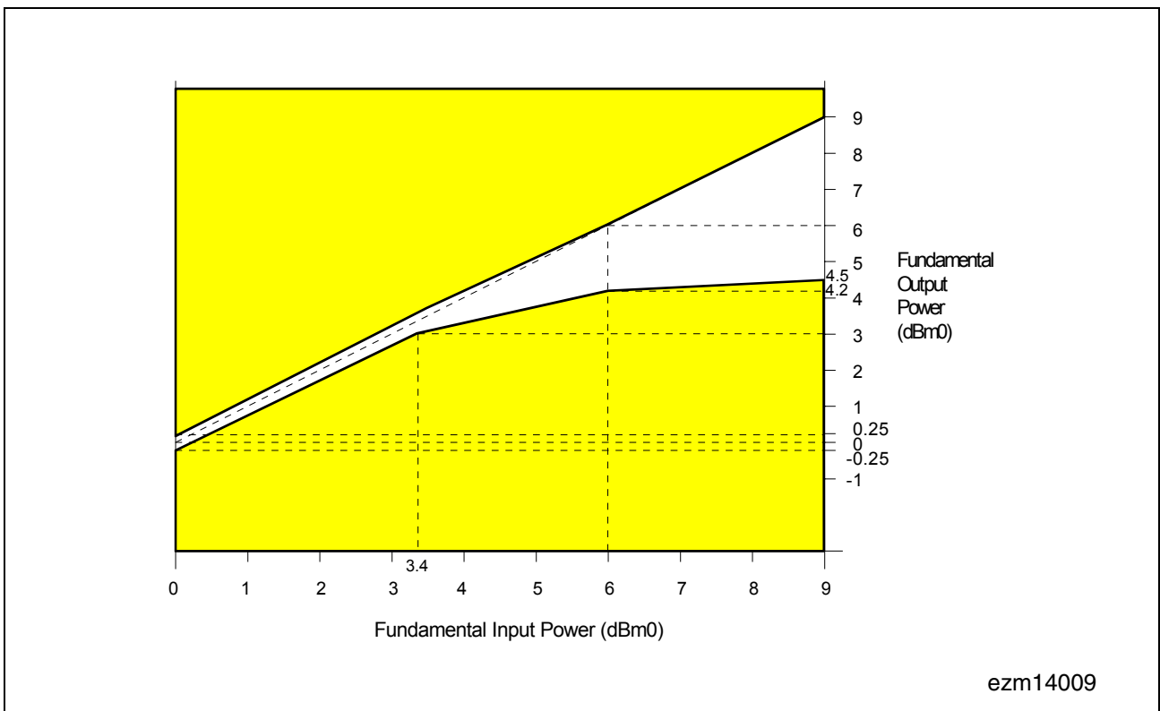
Figure 72 Overload Compression
