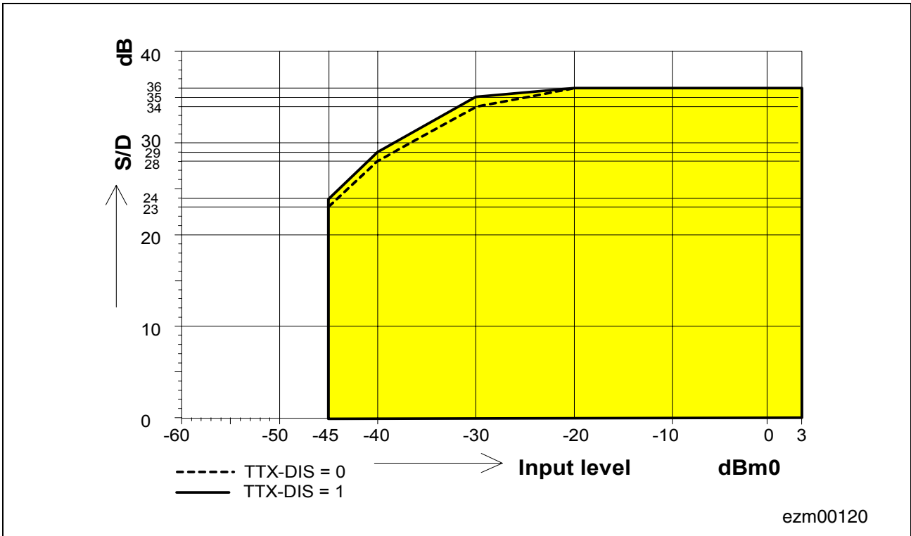
Figure 82 Total Distortion Receive ( L_R = 0 dB)
