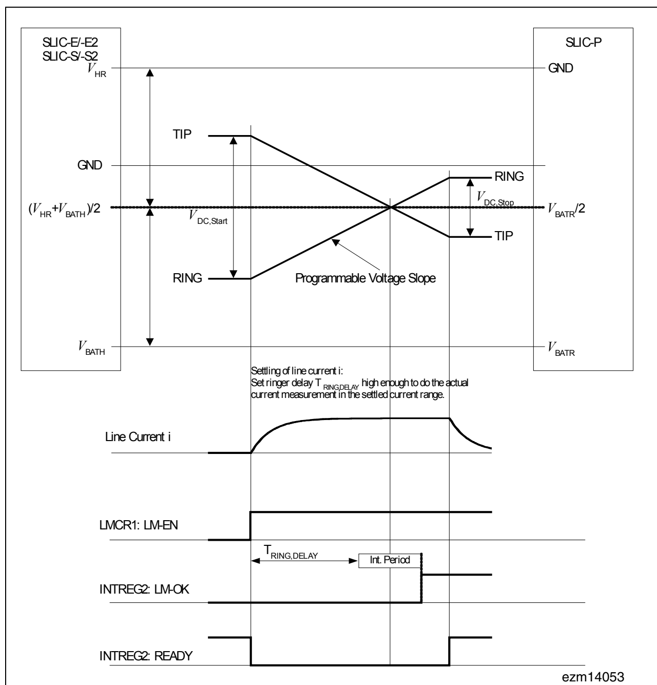
Figure 47 Capacitance Measurement
