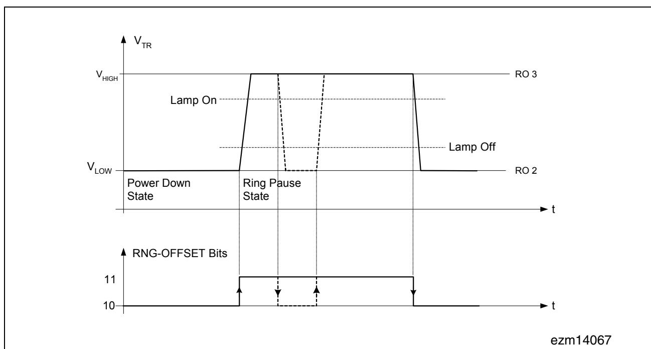
Figure 34 Timing Diagram
