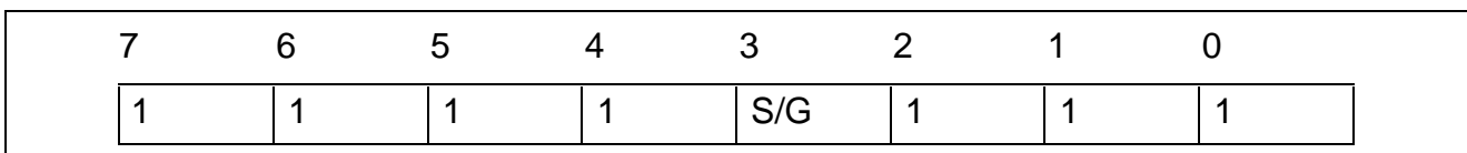
Figure 26 MONITOR Channel on IDP0
