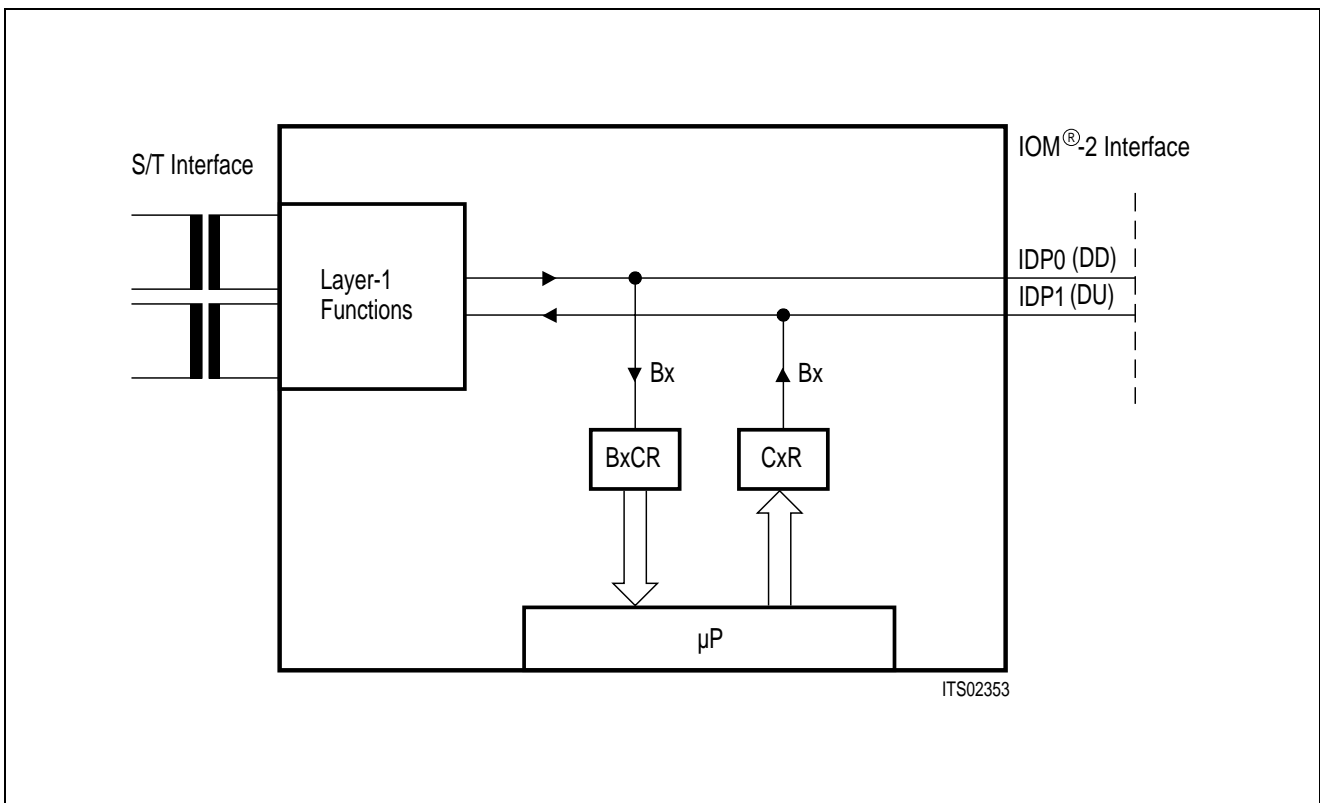
(c) SPCR:CxC1, CxC0 = 10 Bx access from/to S/T transmission of constant value to S/T
