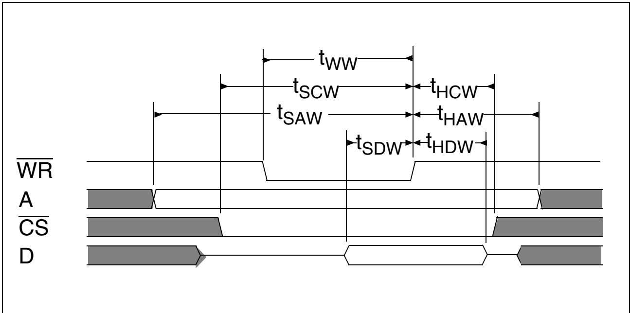
Figure 65 Write Cycle Intel/Infineon Demultiplexed Mode
