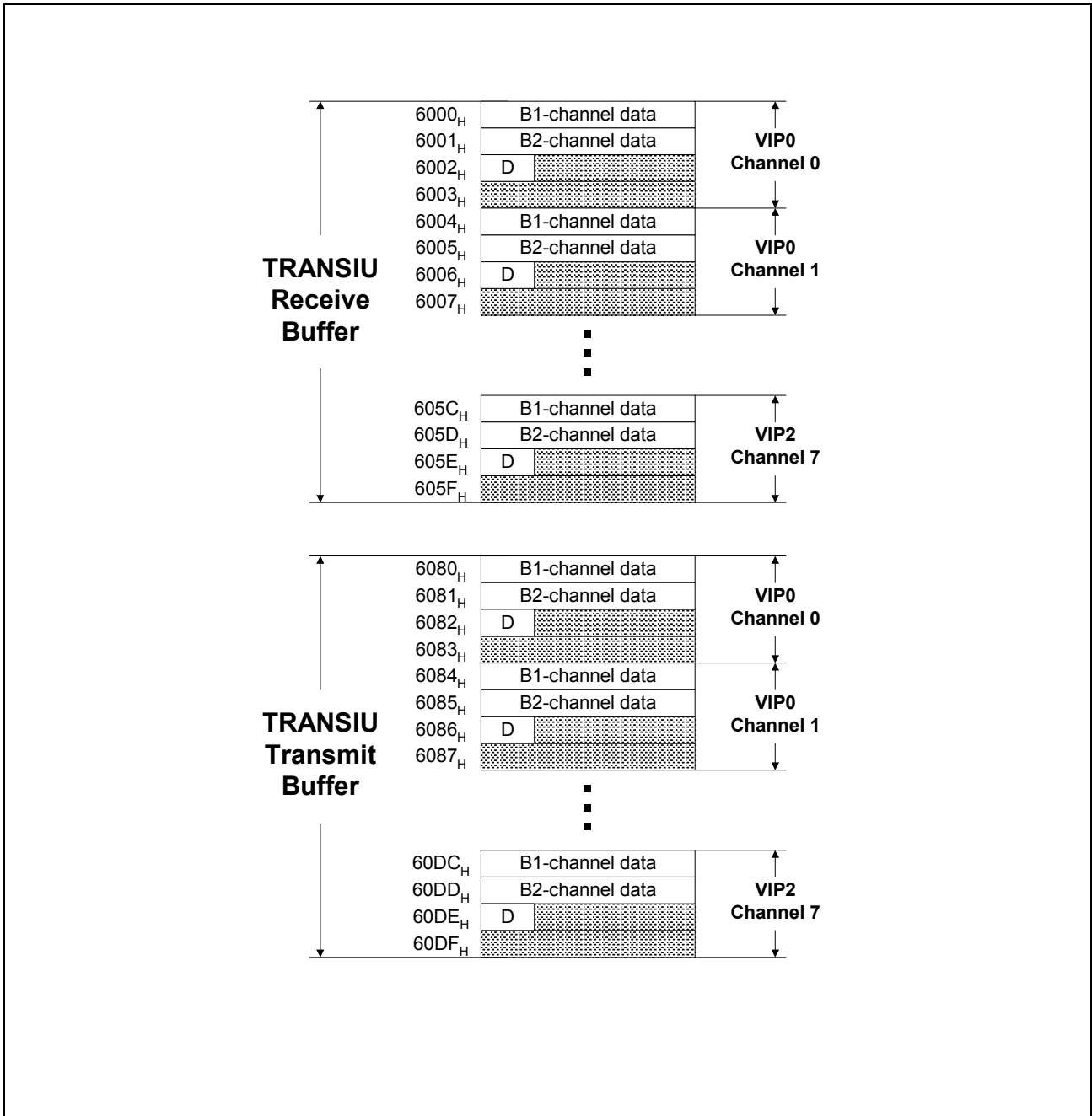
Figure 58 TRANSIU Buffer Addresses
