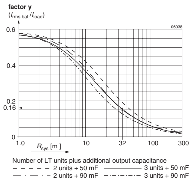
Fig. 12 I_{\text{rms bat}}/I_{\text{load}} versus system resistance ( R_{\text{Sys}} ). 2 and 3 T units in parallel, with additional output capacitors
