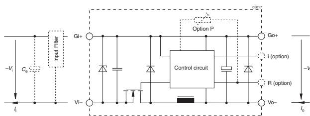
Fig. 3 Single phase configuration L, N 230 V mains: LT-types
