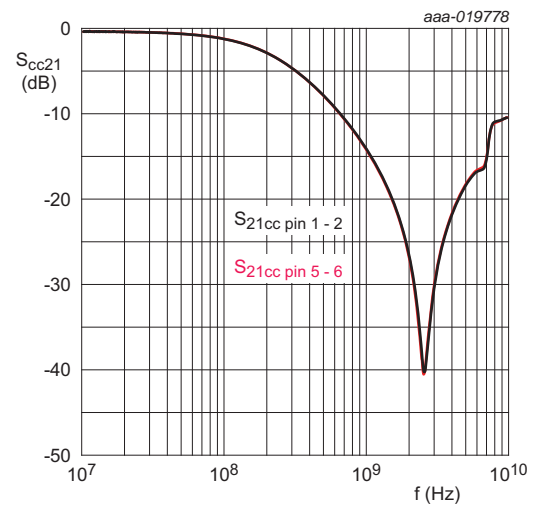
Fig 2. Common-mode insertion loss; typical values
