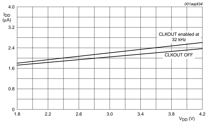
Fig 49. I_{DD} as a function of V_{DD}
