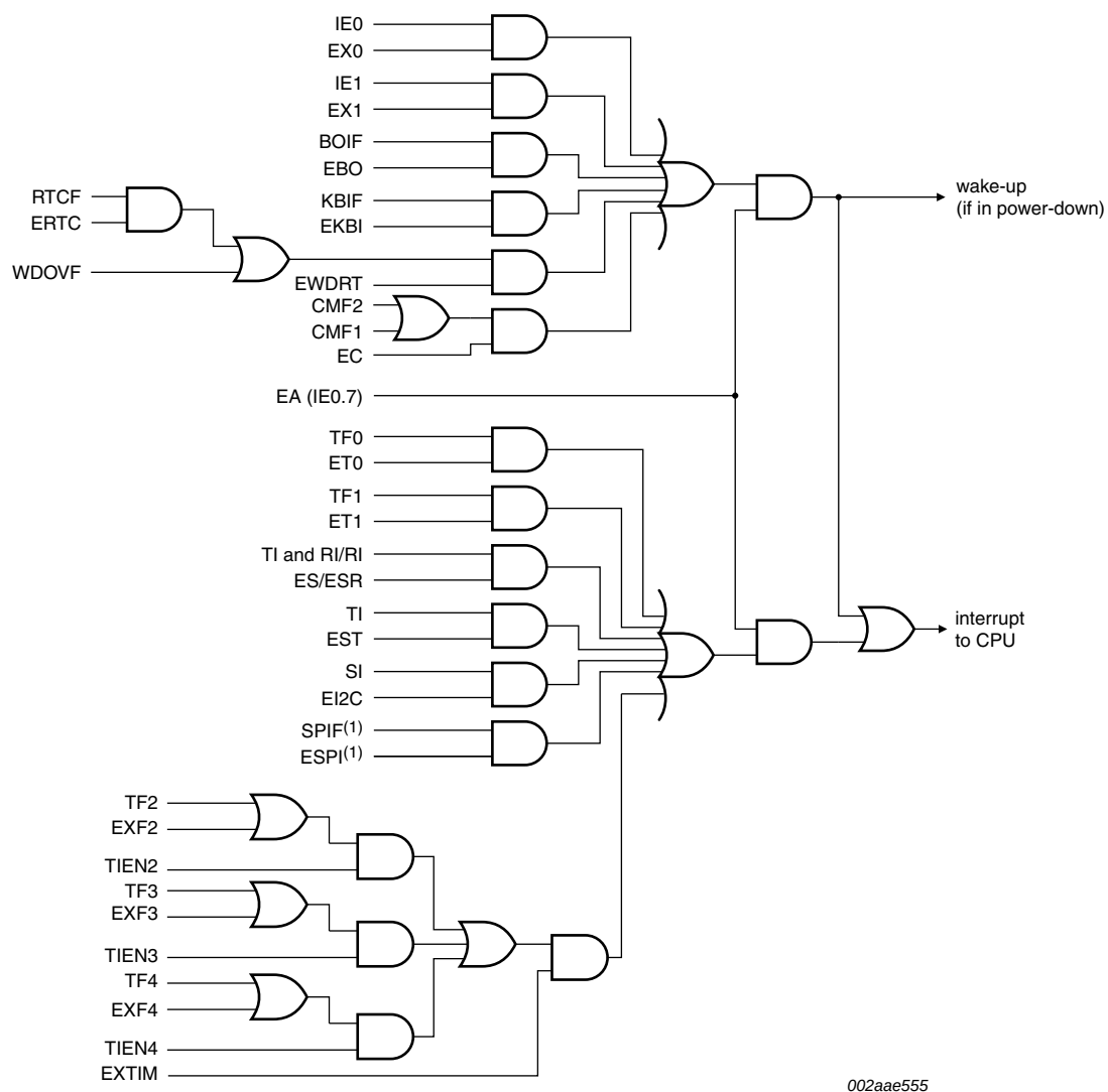
Fig 6. Interrupt sources, interrupt enables, and power-down wake-up sources
