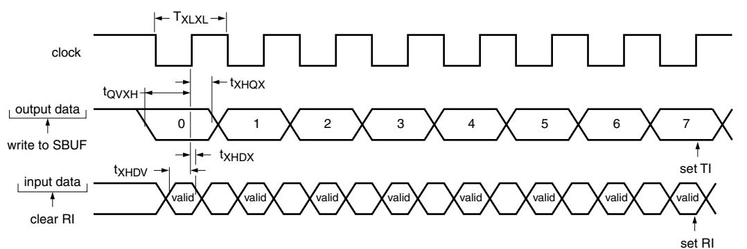
Fig 18. Shift register mode timing
