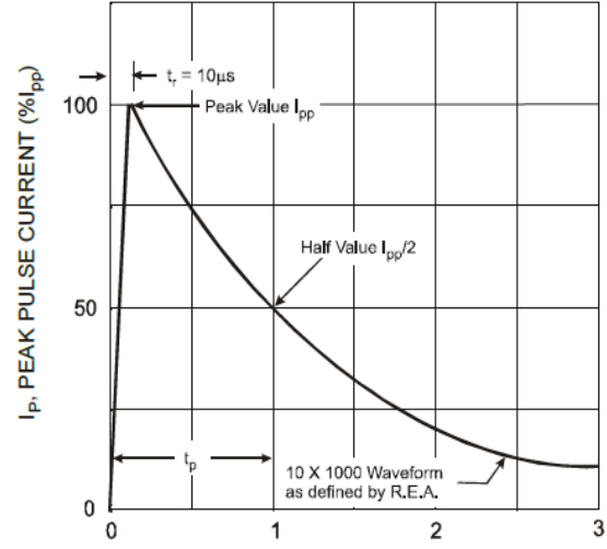
Fig. 4 Pulse Waveform
