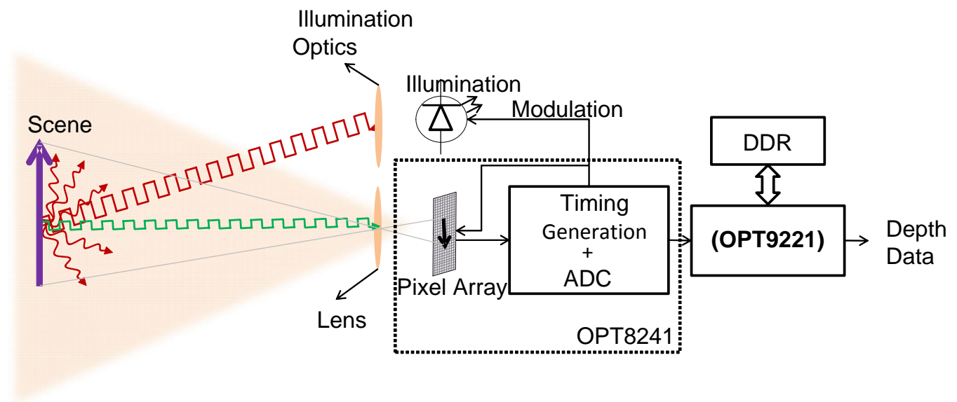
Figure 126. TFC Application Diagram
