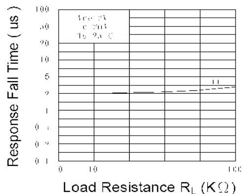
Fig.11 Response Time vs. Load Resistance
