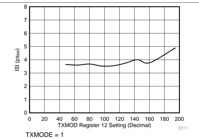
Figure 4. TX Deterministic Jitter vs Modulation Current
