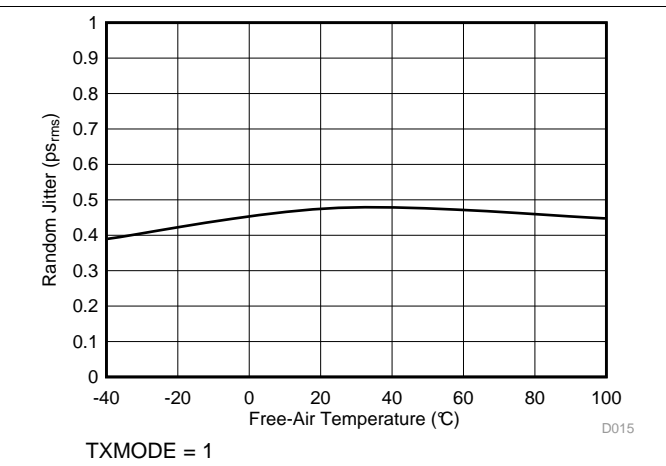
Figure 8. TX Random Jitter vs Temperature
