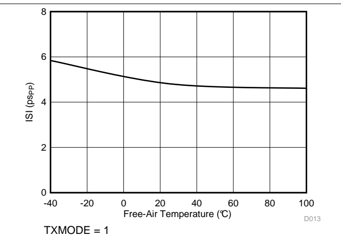
Figure 6. TX Deterministic Jitter vs Temperature
