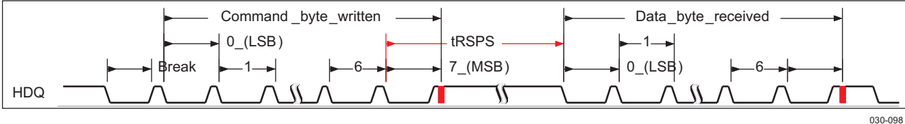
Figure 6-58. HDQ Communication Timing
