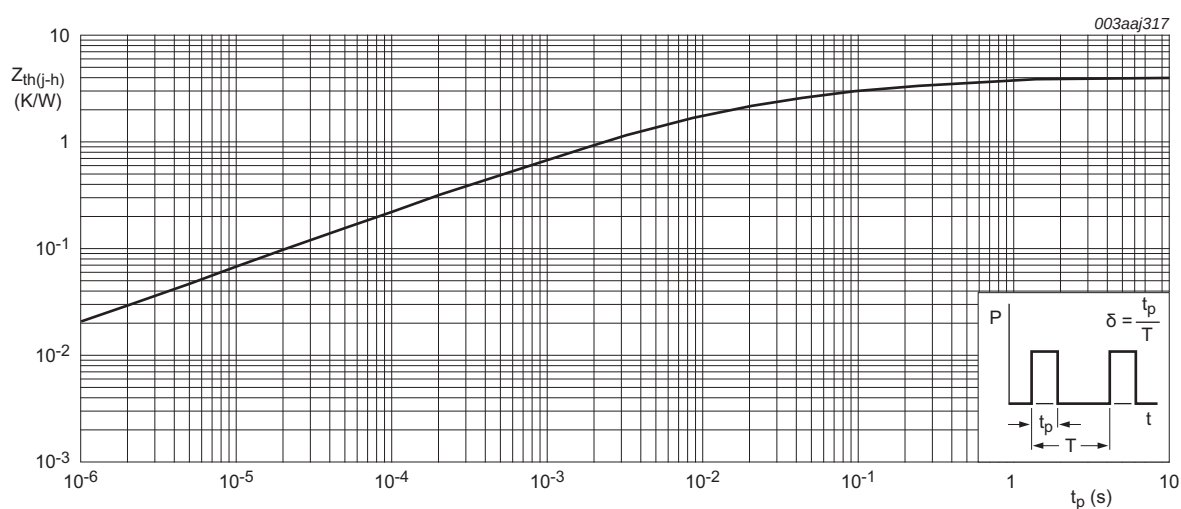
Fig 5. Transient thermal impedance from junction to heatsink as a function of pulse width; per diode
