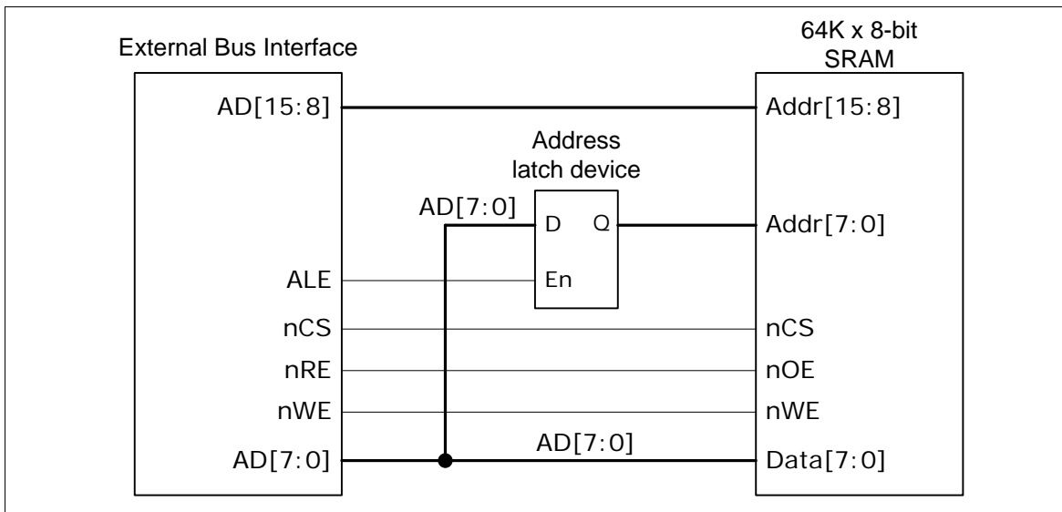
Figure 5-113 Connection of 8-bit EBI Data Width with 8-bit Device
