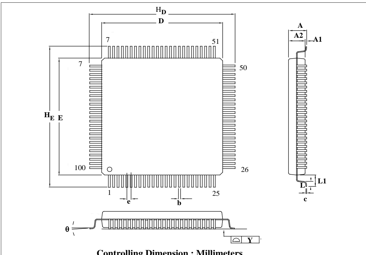
Controlling Dimension : Millimeters
