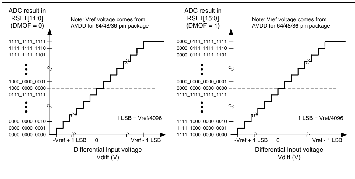
Figure 5-107 ADC Differential Input Conversion Voltage and Conversion Result Mapping Diagram
