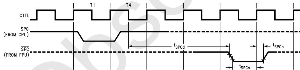
FIGURE 4-12. \overline{SPC} Timing
