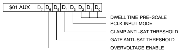
Figure 13. AUX Register Bit Definitions
