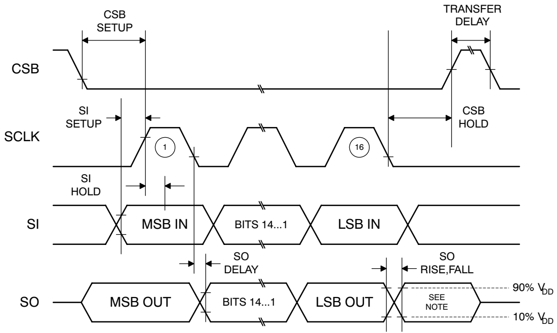
Figure 9. SPI Timing
