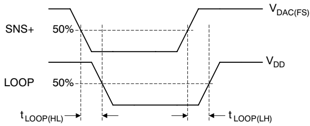
Figure 3. LOOP Output Response Delay
