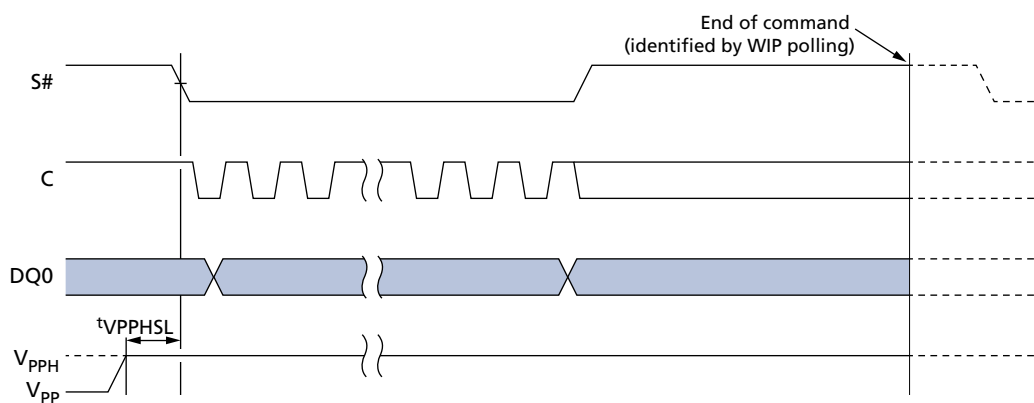
Figure 46: V_{PPH} Timing
