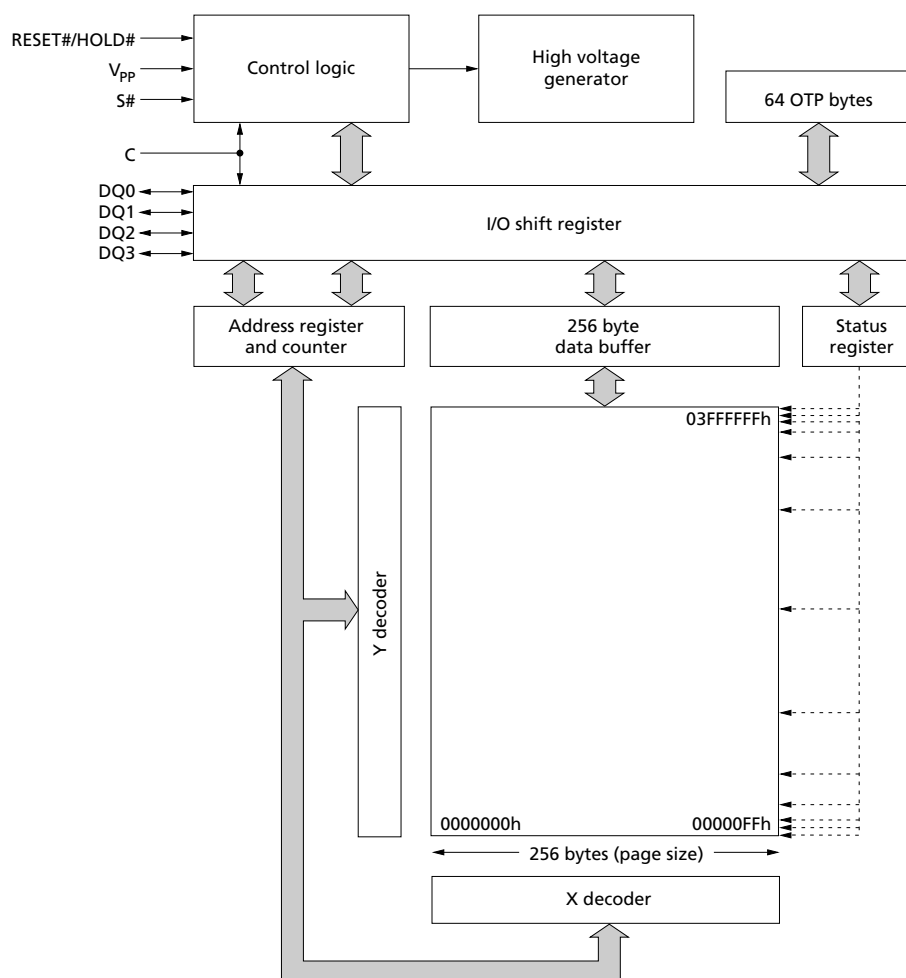
Figure 5: Block Diagram
