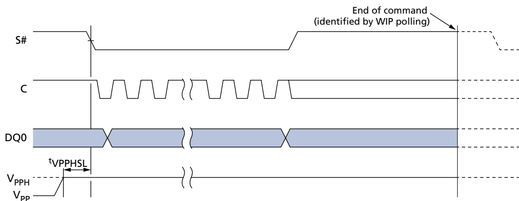
Figure 38: V_{PPH} Timing
