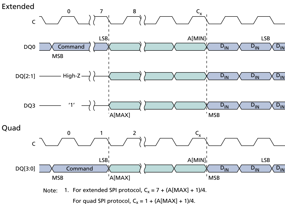
Figure 29: EXTENDED QUAD INPUT FAST PROGRAM Command
