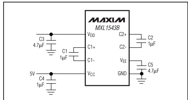
Figure 10. Charge Pump
