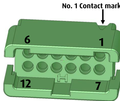
Male Crimp Housing
