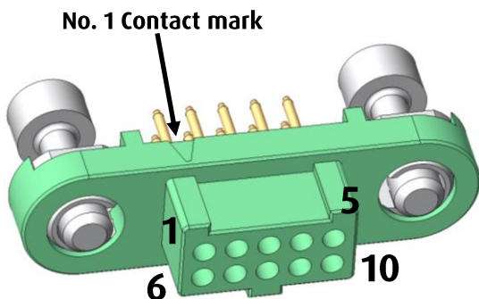
Female PCB mounted
