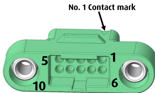
Male Crimp Housing
