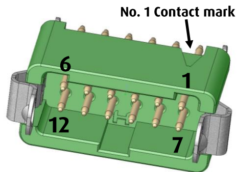
Male PCB mounted
