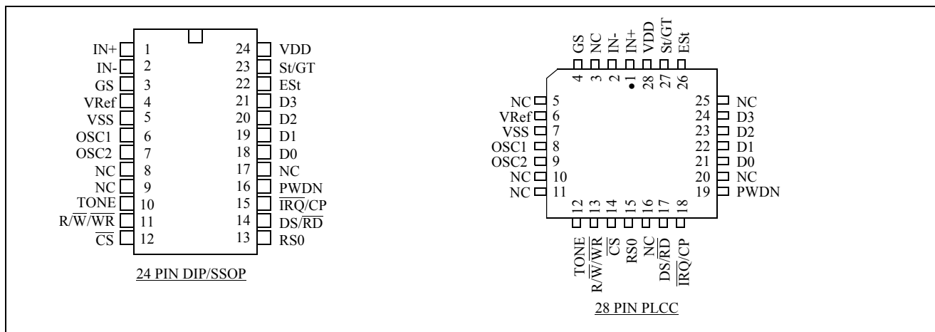
Figure 2 - Pin Connections
