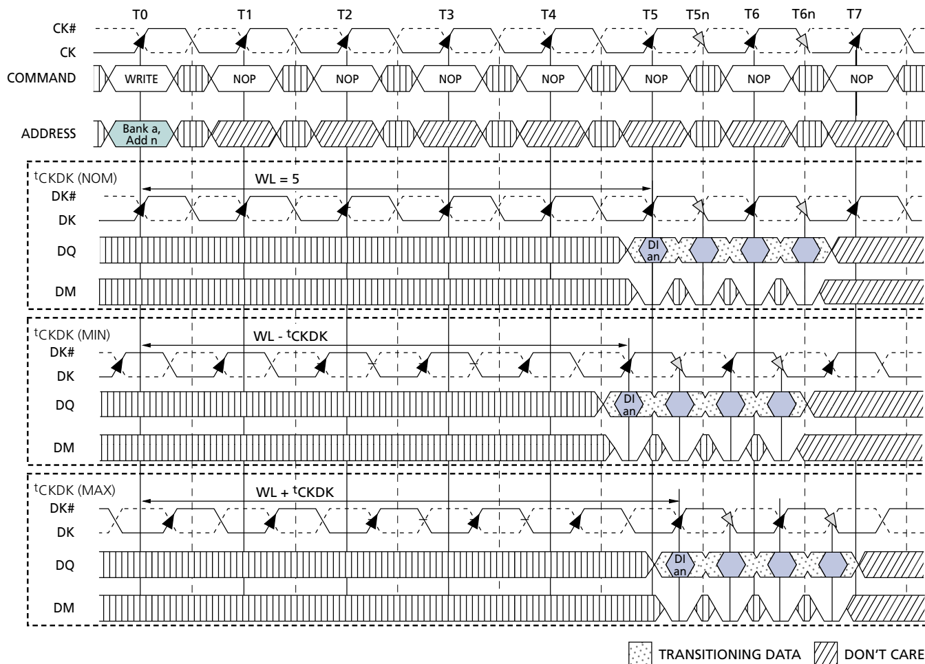
Figure 29: WRITE Burst
