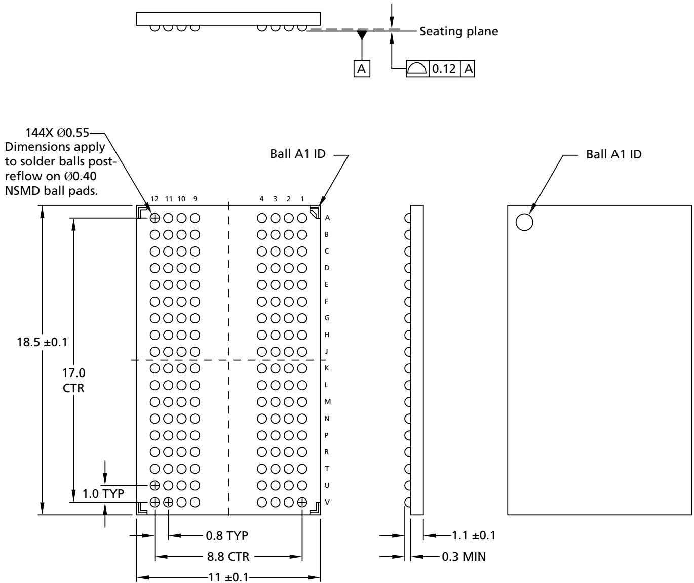
Figure 7: 144-Ball FBGA
