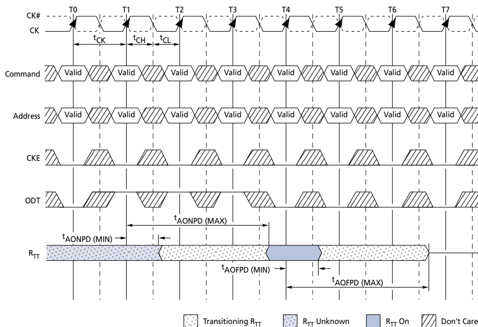
Figure 84: ODT Turn-Off Timings When Entering Power-Down Mode
