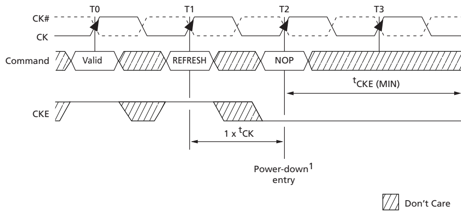
Figure 77: REFRESH Command-to-Power-Down Entry
