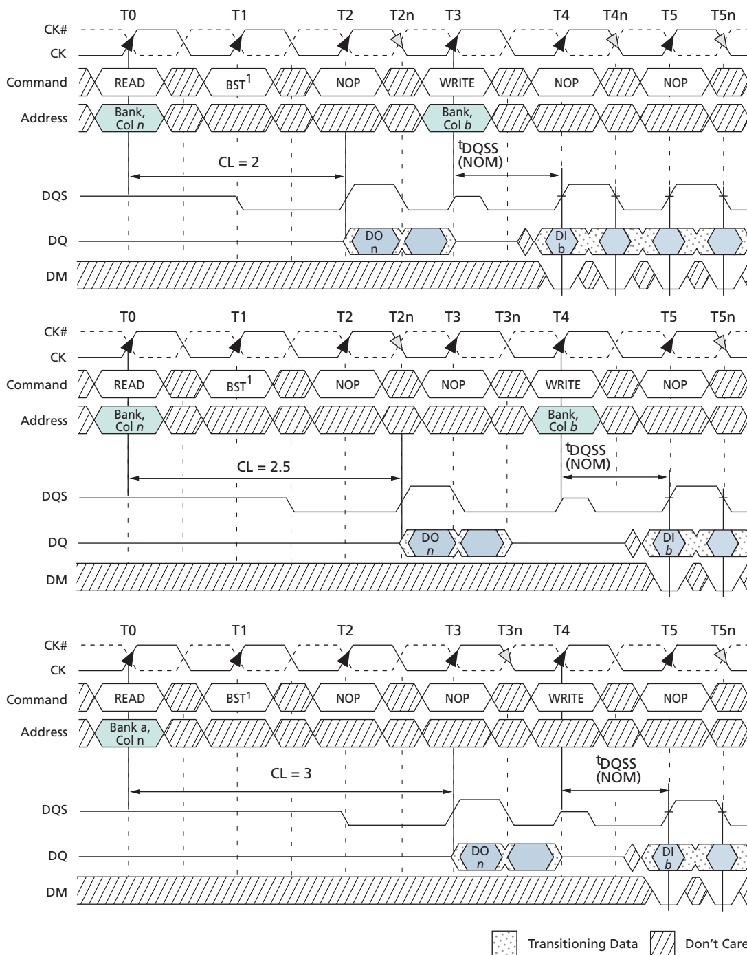
Figure 30: READ-to-WRITE
