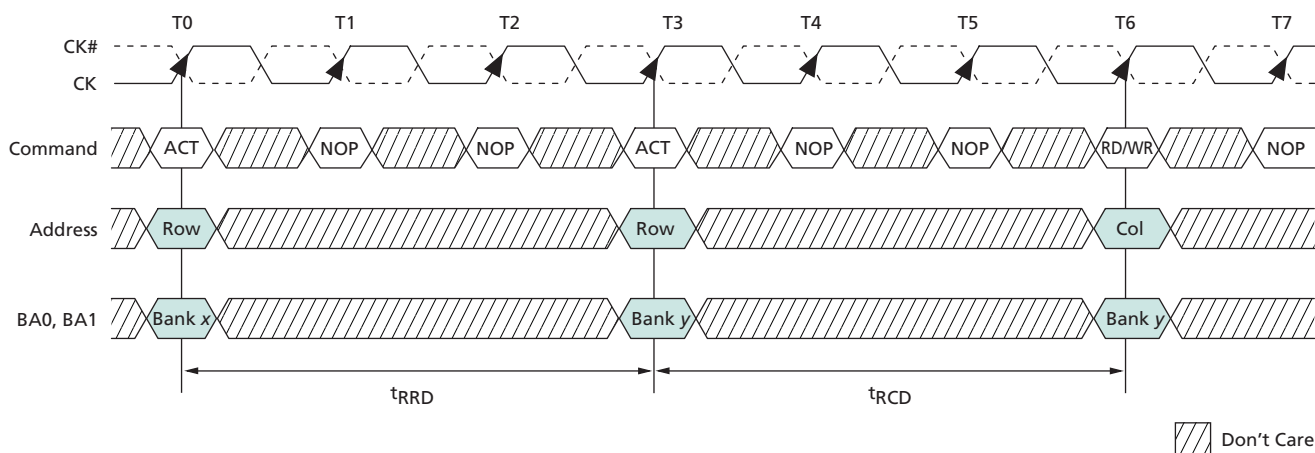
Figure 24: Example: Meeting t_{\text{RCD}} ( t_{\text{RRD}} ) MIN When 2 < t_{\text{RCD}} (t_{\text{RRD}}) \text{ MIN} / t_{\text{CK}} \leq 3
