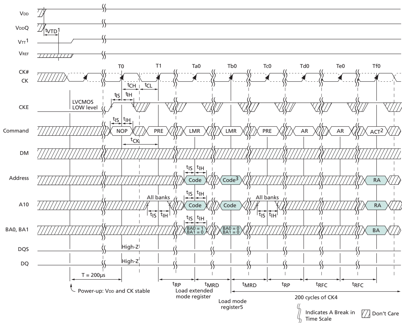
Figure 22: INITIALIZATION Timing Diagram
