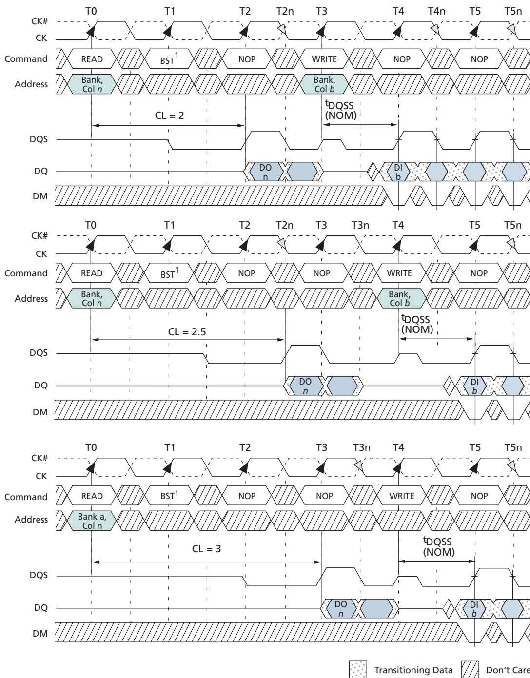
Figure 32: READ-to-WRITE
