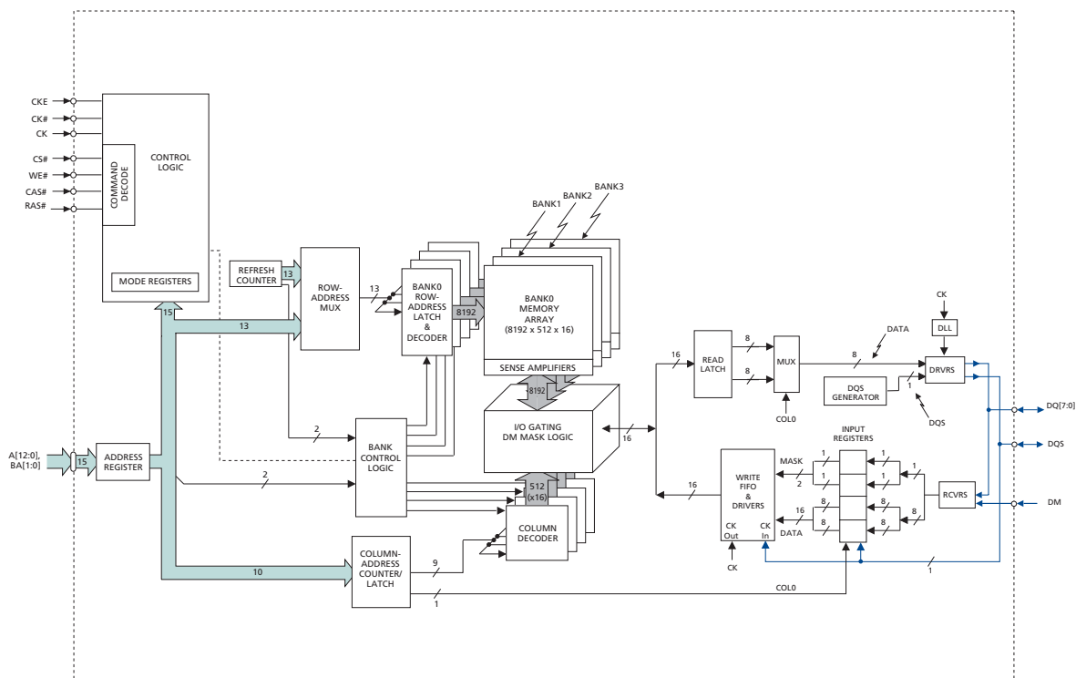
Figure 4: 32 Meg x 8 Functional Block Diagram
