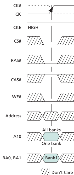
Figure 20: PRECHARGE Command
