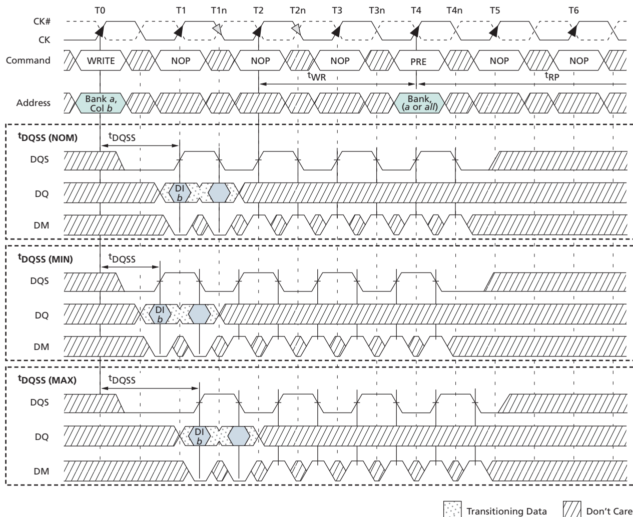
Figure 46: WRITE-to-PRECHARGE – Interrupting
