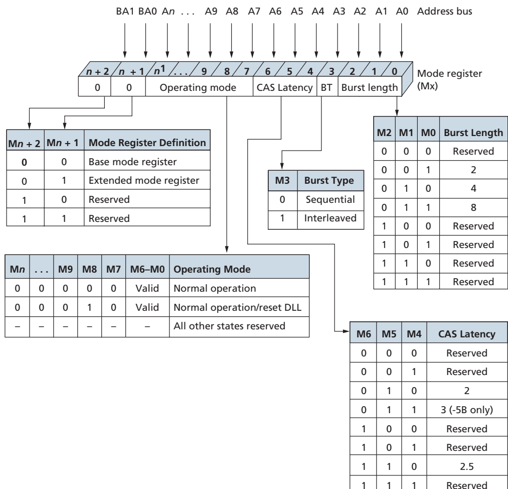
Figure 21: Mode Register Definition
