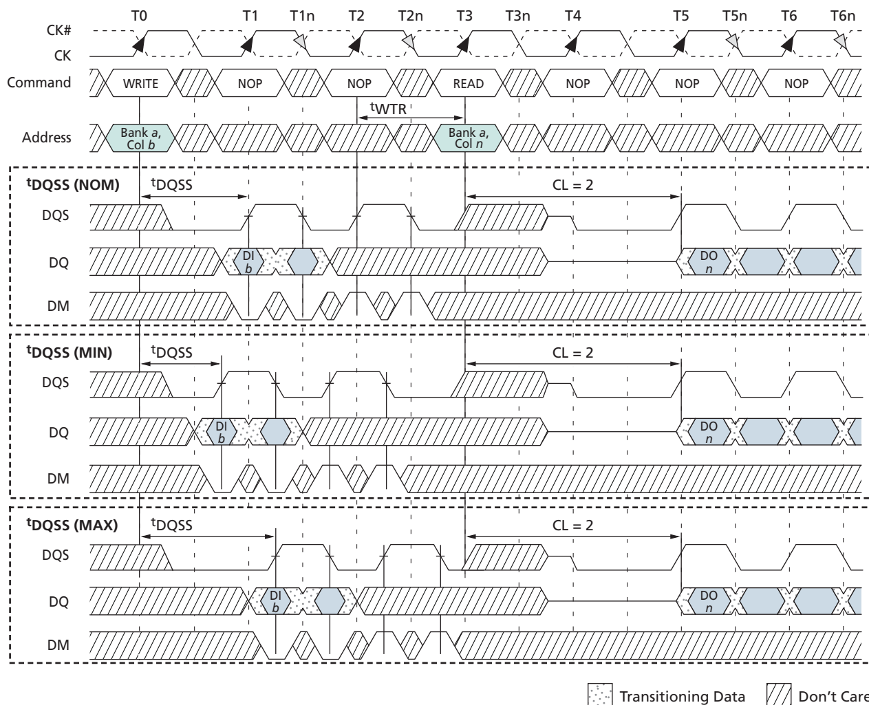
Figure 41: WRITE-to-READ – Interrupting
