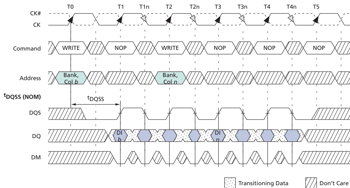
Figure 37: Consecutive WRITE-to-WRITE
