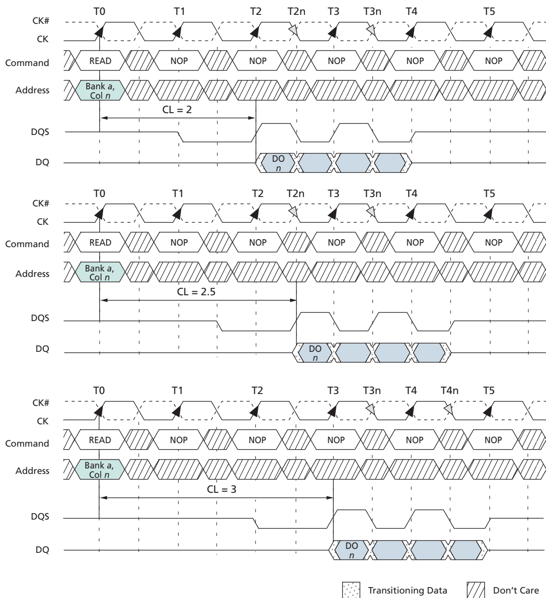
Figure 25: READ Burst
