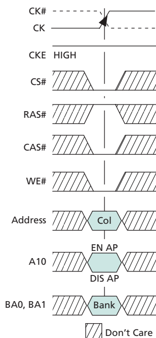
Figure 17: WRITE Command
