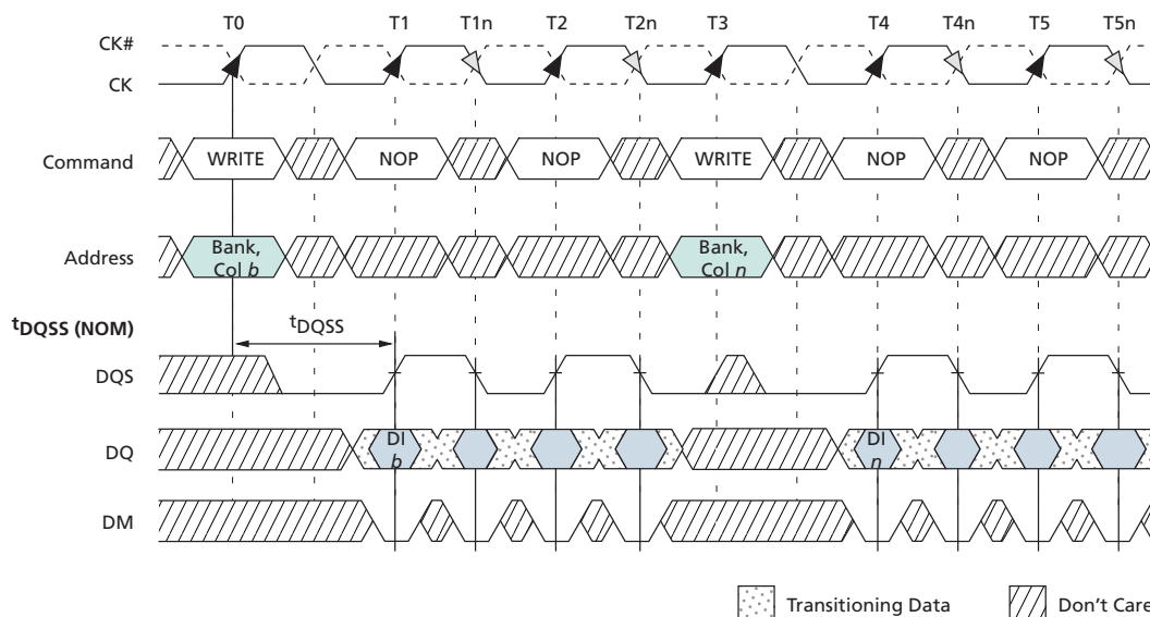
Figure 38: Nonconsecutive WRITE-to-WRITE
