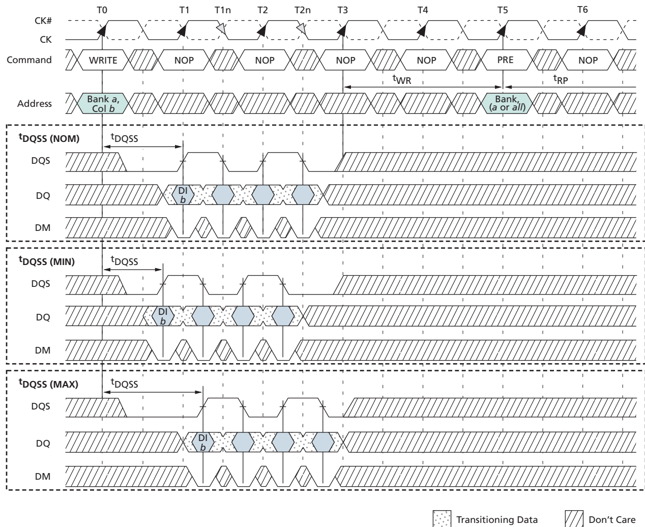
Figure 46: WRITE-to-PRECHARGE – Uninterrupting
