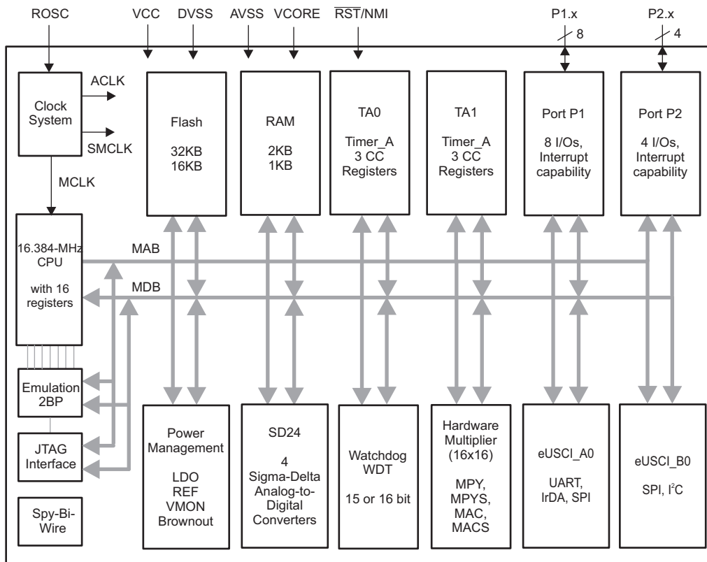
Figure 6-2. Functional Block Diagram – PW Package – MSP430i2041, MSP430i2040
