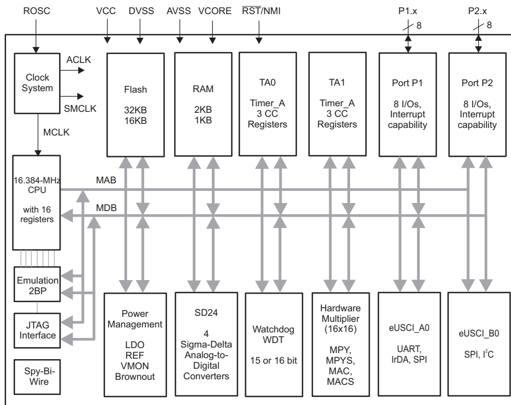
Figure 1-1. Functional Block Diagram – RHB Package – MSP430i204x
