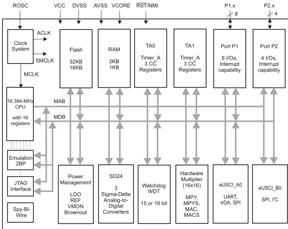
Figure 6-4. Functional Block Diagram – PW Package – MSP430i2031, MSP430i2030
