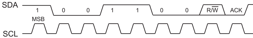
Figure 9. Slave Address
