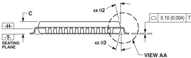
VIEW AA
