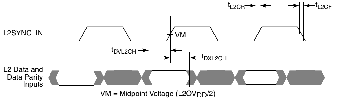
Figure 8. L2 Bus Input Timing Diagrams
