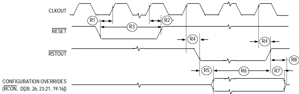
Figure 22-7. \overline{\text{RESET}} and Configuration Override Timing
