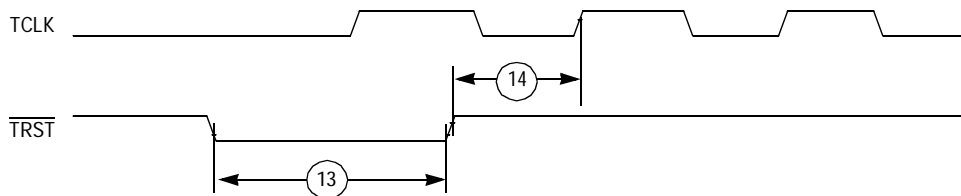
Figure 22-12. \overline{TRST} Timing
