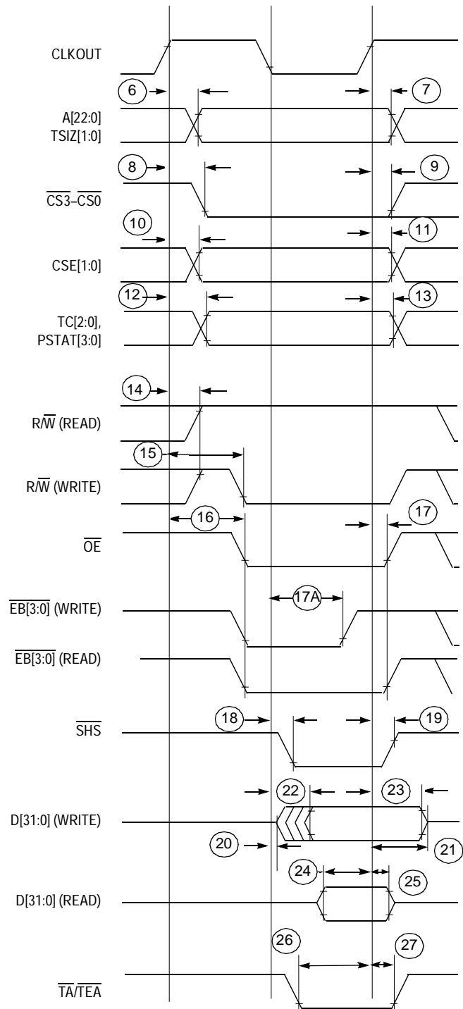
Figure 22-4. Clock Read/Write Cycle Timing
