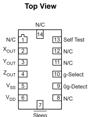
Figure 4. Pinout Description
