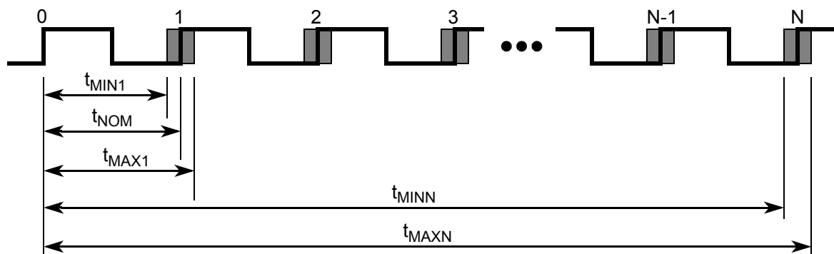
Figure 10. Jitter Definitions
