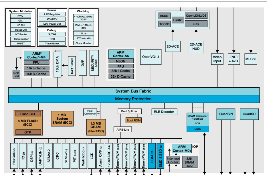
MAC57D5xx Block Diagram
