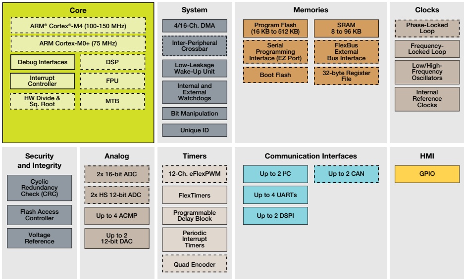
Kinetis V Series MCU Family Block Diagram
