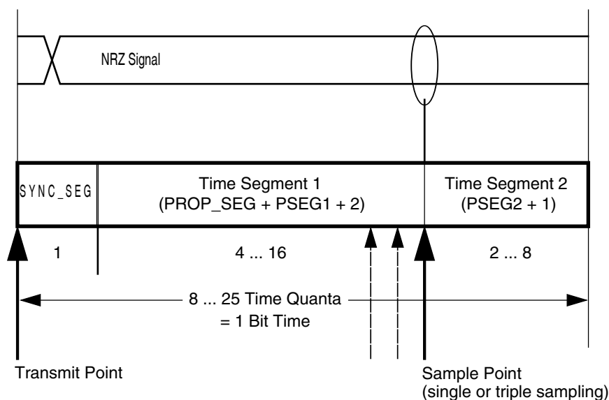
Figure 48-105. Segments within the Bit Time
