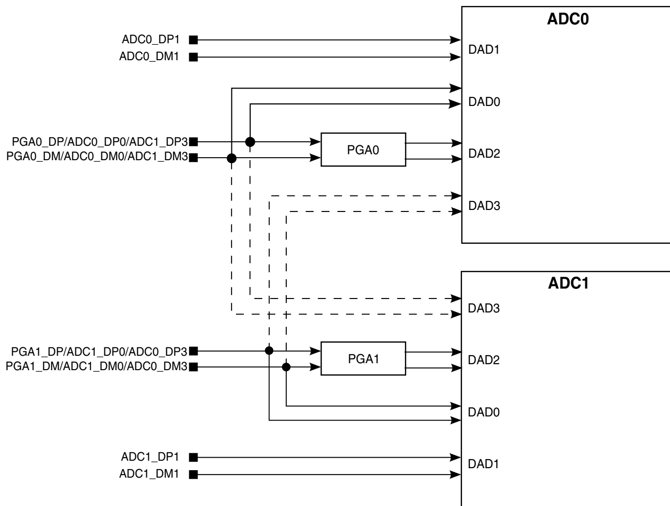
Figure 3-39. PGA Integration
