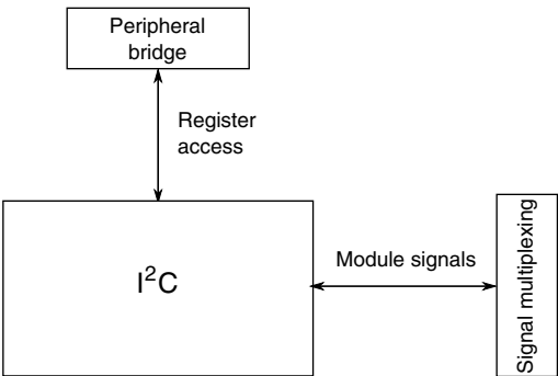
Figure 3-61. I2C configuration
