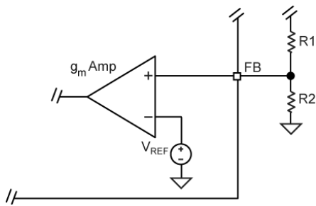
Figure 6. Voltage-Divider Configuration
