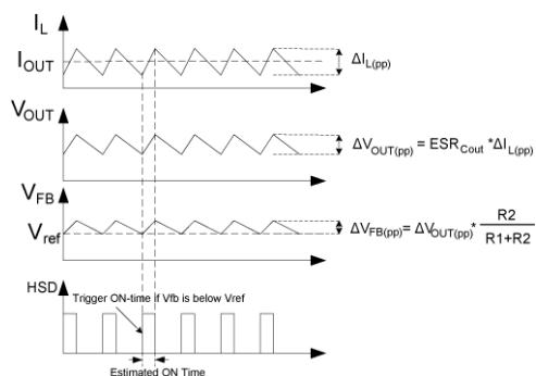
Figure 2. MIC26601 Control Loop Timing
