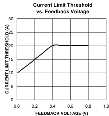
Figure 5. MIC261203 Current-Limit Foldback Characteristic
