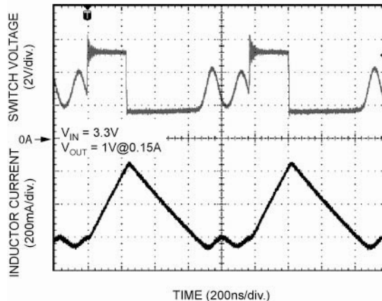
Discontinuous Operation
