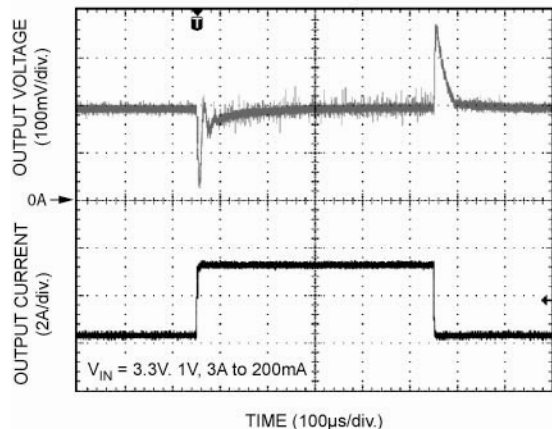
Transient Response
