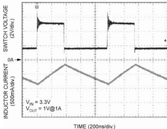
Continuous Operation
